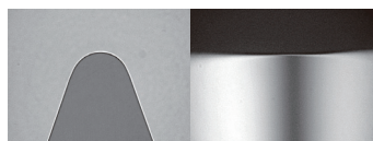
刃先拡大写真 Macro photograph of cutting edge tip
