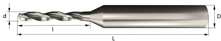
Style C | Carbide 3-Flute Twist Drill with Reinforced Shank
