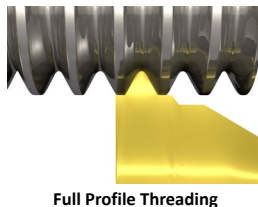
Full Profile Threading
